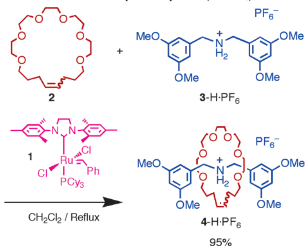
Scheme 1. Magic Ring Synthesis of a [2]Rotaxane ( 4 ·H·PF 6 ) Templated by a Linear Ammonium Ion-Containing Dumbbell-Shaped Component ( 3 ·H·PF 6 )
