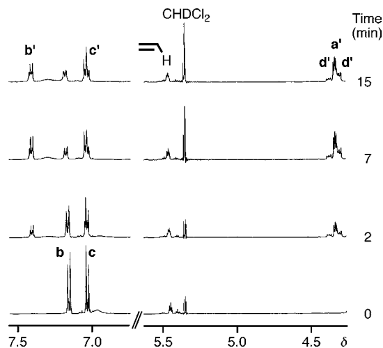
Figure 1. Partial 1 H NMR spectra showing the change over time during the magic ring synthesis of the dynamic [2]catenane 11-H·PF 6 . Peak labels are defined in Scheme 3.
