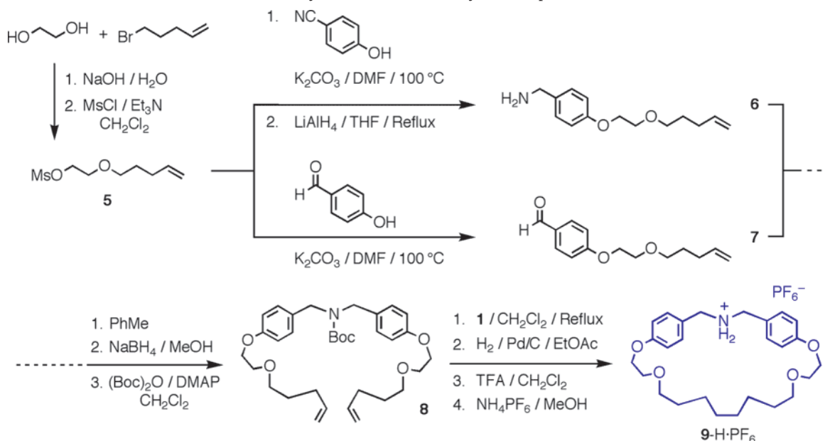
Scheme 2. Synthesis of the Macrocyclic Template 9 ·H·PF 6
