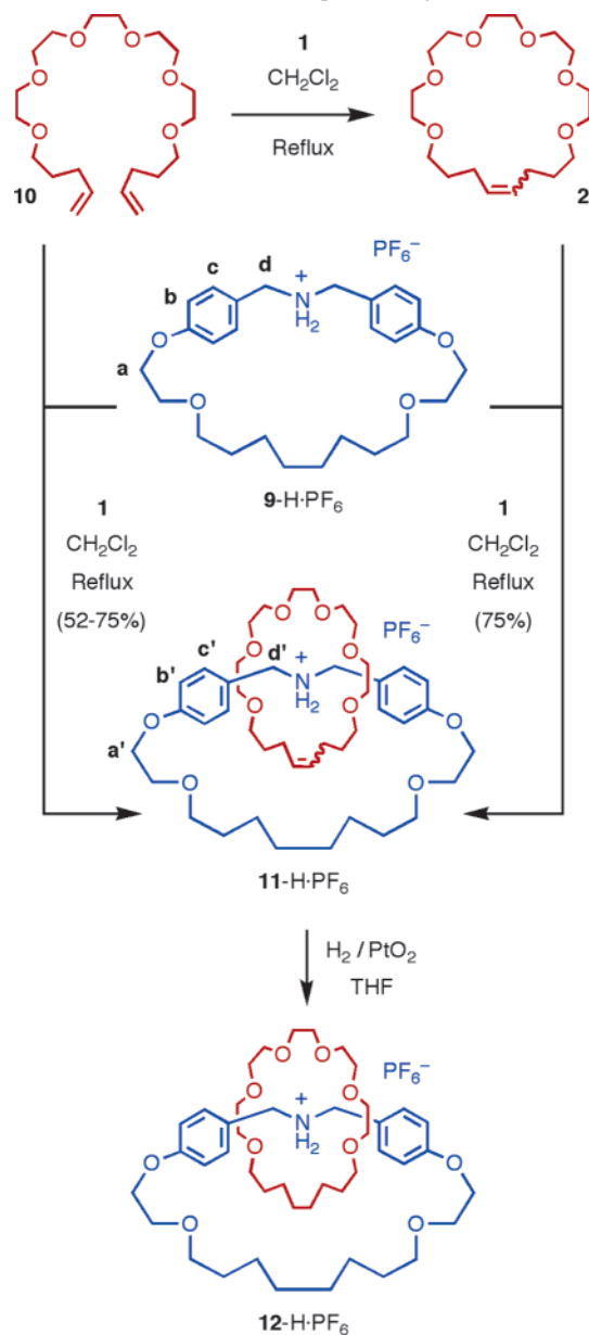
Scheme 3. Dynamic Synthesis of a Catenane ( 11-H·PF 6 ) by Two Distinct, Yet Complementary, Routes a
